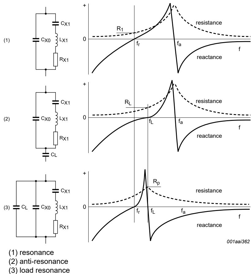
Fig. 13. Reactance and resistance characteristics of a crystal
