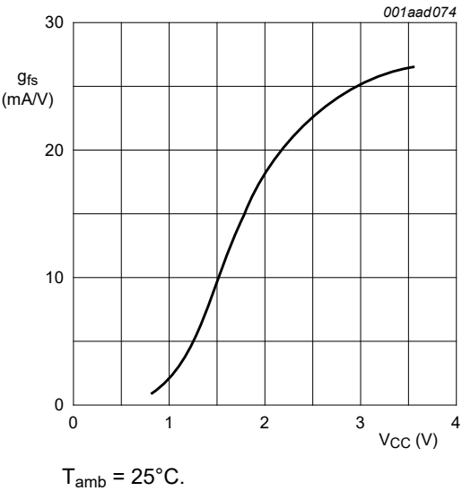
Fig. 11. Typical forward transconductance as a function of supply voltage
